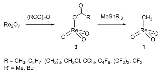
Scheme 2. Synthesis of MTO with mixed anhydrides of perrhenic acid. [15]
