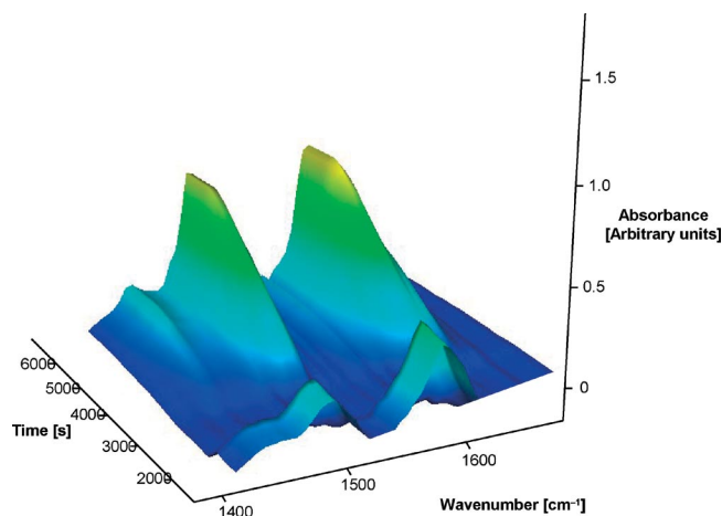
Figure 1. In situ IR spectra for the synthesis of methylzinc acetate from the reaction of zinc acetate with trimethylaluminum.
