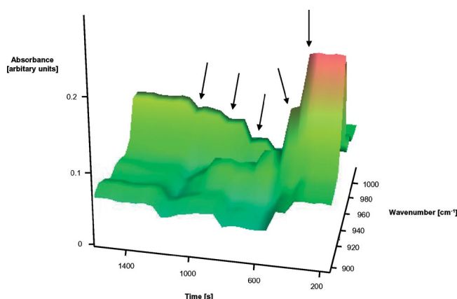
Figure 3. Series of IR spectra obtained from the reaction of acetyl perrhenate with methylzinc acetate (successive addition of small portions of methylzinc acetate is indicated by black arrows). MTO shows a pronounced vibration at 961 cm -1 .
