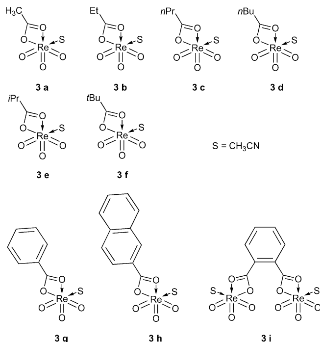
Scheme 4. Selected set of perrhenyl carboxylates 3a–i .
