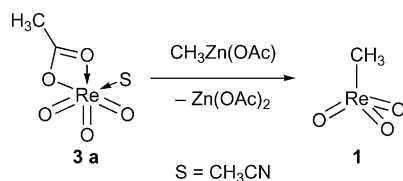
Scheme 3. Synthesis of MTO with the use of acetyl perrhenate and methylzinc acetate. [20]
