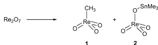
Scheme 1. The first literature reported multigram-scale synthesis of methyltrioxorhenium. [5]
